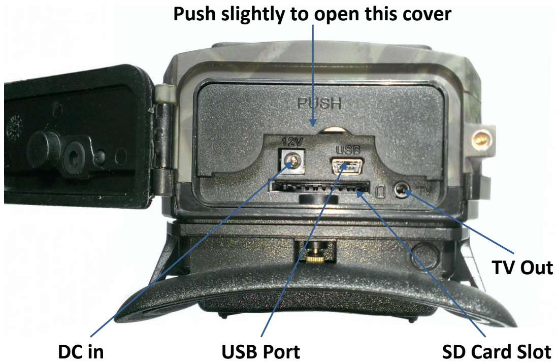
2.2 Figure 3.2: Bottom View of Camera;
